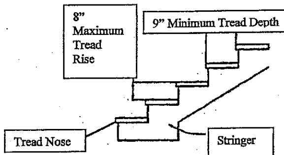
STAIR DESIGN DETAIL (NOT TO SCALE)
