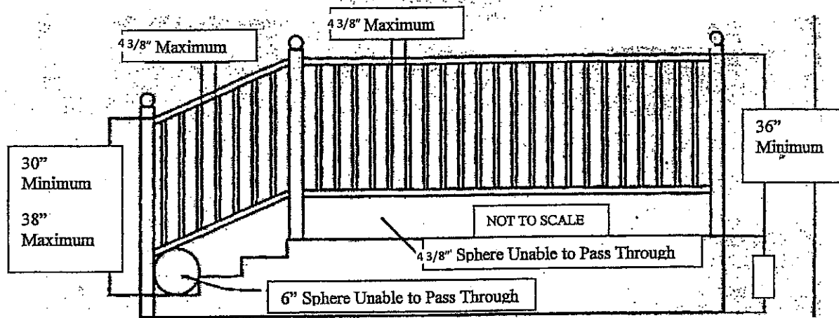
HANDRAILS, GUARDRAILS & STAIRS (NOT TO SCALE)
